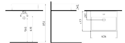
INFINITIUM COUNTERTOP WB. 60 CM SINGLE HOLE INLG06001FD1W5000 600mm
