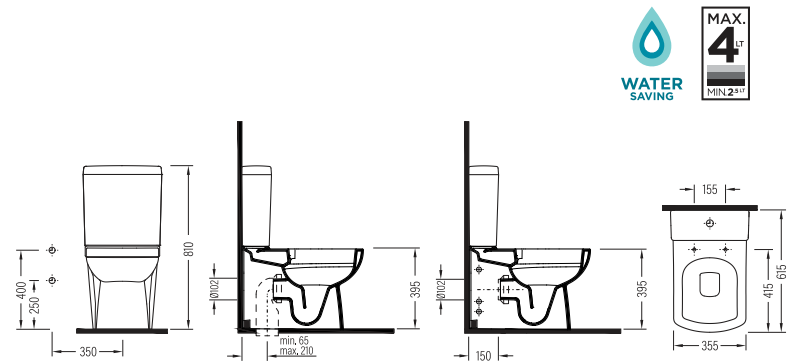
BACK TO WALL CLOSE COUPLED WC PAN 62 CM NO-RIM GYKD062N1VPOW5000
