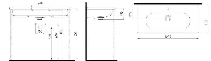
VANITY WASHBASIN 100 cm SINGLE HOLE FELK10001FD1W5000 1000x465mm
