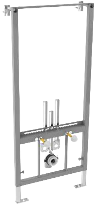
SUPREME FRA-B SANITARY INSTALLATION FRAME FOR BIDETS FRFDBD00000B0
