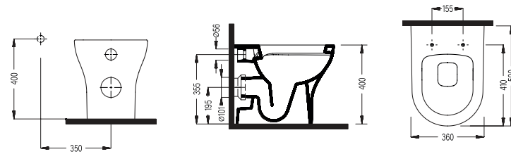
ROOT BTW WC PAN 50 CM WITHOUT BIDET FUNCTION COOL WHITE EXT. ROKK05001VP0W5SZ0
