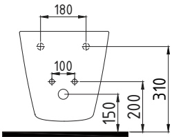
WALL HUNG BIDET 54 cm SINGLE HOLE ALBA05401VD1W5000 540x360mm
