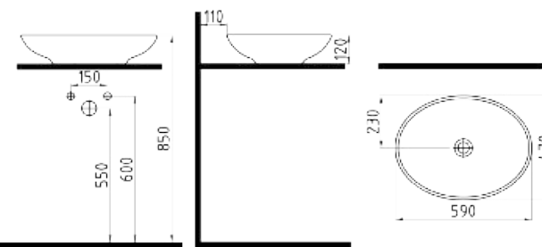
COUNTERTOP WASHBASIN 59 cm WITHOUT HOLE HRLG05901FDOW5000 590x470mm
