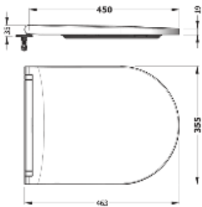
VENTO ELITE UF/ DUROPLAST AB SOFTCLOSE EASYRELEASE SEAT COVER
