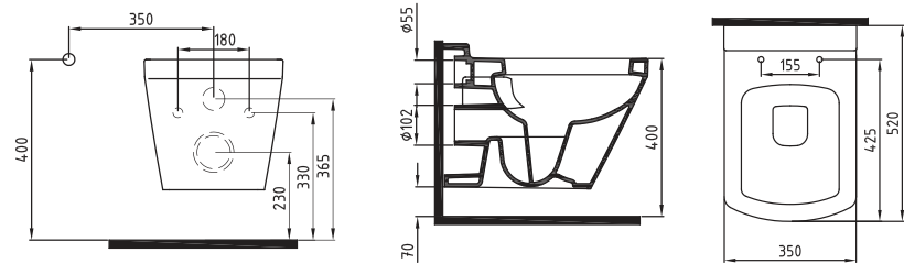
NEPTUN WALL HUNG WC PAN 52 cm NPKA052AMVPOW5000 520x350mm
