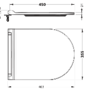
VENTO MONOSLIM UF/DUROPLAST AB SOFTCLOSE EASYRELEASE SEAT COVER
