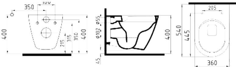
WALL HUNG WC PAN 54 cm NO-RIM CONCEALED FIXING ALKA054N1VP0W5000 540x360mm
