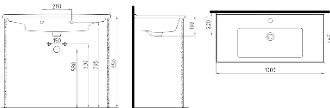
VANITY WASHBASIN 100 cm SINGLE HOLE NPLK10001FD1W5000 1000x470mm
