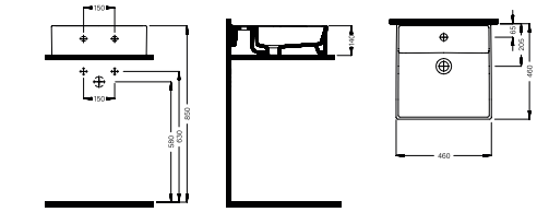
INFINITIUM COUNTERTOP WB. 46 CM SINGLE HOLE INLG04601FD1W5000 460mm
