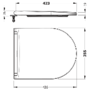
RICO ELITE UF/ DUROPLAST AB SOFTCLOSE EASYRELEASE SEAT COVER
