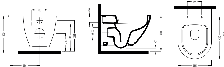
WALL HANG WC PAN 52 CM NO-RIM NCKA052N2VP1W5000 520x355 mm
