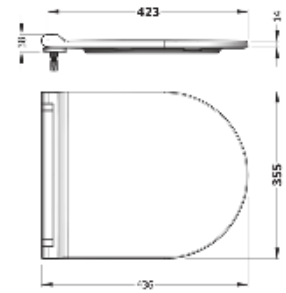
RICO MONOSLIM PROPLAST SOFTCLOSE EASYRELEASE SEAT COVER
