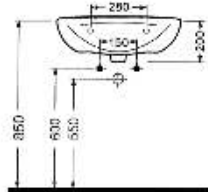
SINGLE PIECE DISABLED WASHBASIN 60 cm SINGLE HOLE TPLE06001VD1W5000 600x510mm
