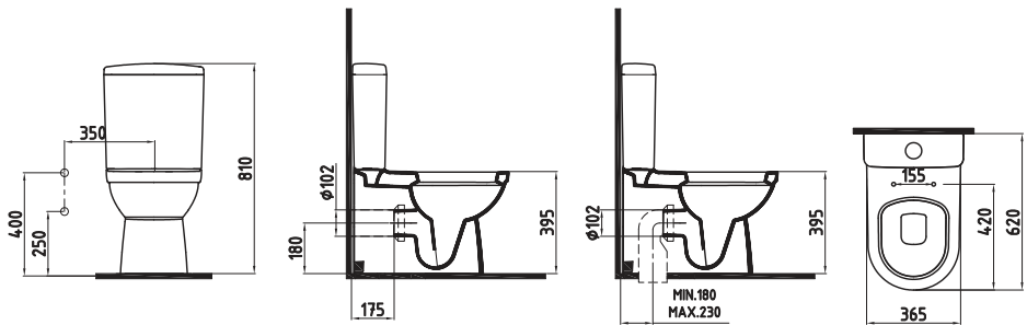
CISTERN 41 cm BOTTOM INLET CPRS04101VD4W5000 410x370mm
