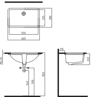
UNDER COUNTER WASHBASIN 53 cm WITHOUT HOLE ROSE GOLD DECOR FALG05301FD009SZ0 550x325mm
