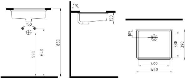
INFINITUM UNDERCOUNTER WASHBASIN 40 cm WITHOUT HOLE INLA04001FDOW5000
