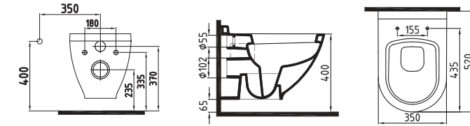
WALL HUNG WC PAN 52 cm HRKA052AMVP0W5000 520x350mm
