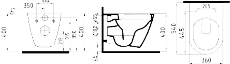
WALL HUNG WC PAN 54 cm NO-RIM CONCEALED FIXING ALKA054N1VP0W5000 540x360mm
