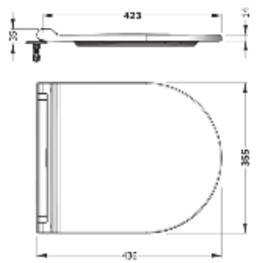
RICO MONOSLIM UF/DUROPLAST AB SOFTCLOSE EASYRELEASE SEAT COVER
