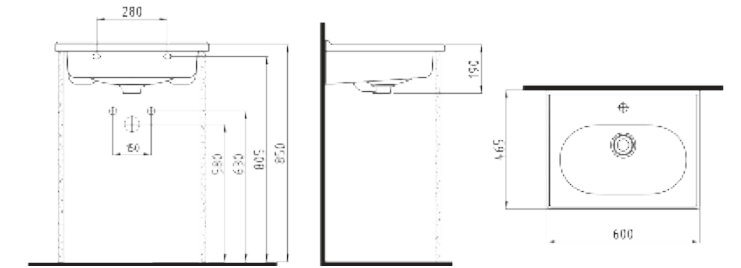
VANITY WASHBASIN 60 cm SINGLE HOLE FELK060B1FD1W5000 600x465mm
