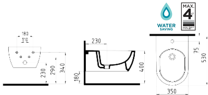
WALL HUNG BIDET 52 cm N3 SINGLE HOLE HRBA05203VD1W5000 530x350mm
