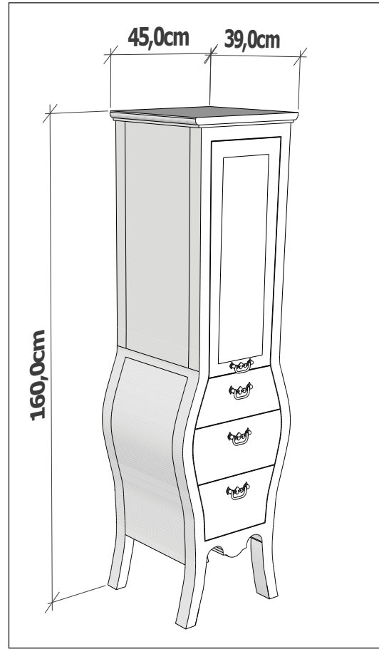
ARIA MINIMAL BOY DOLABI Tall cabinet
